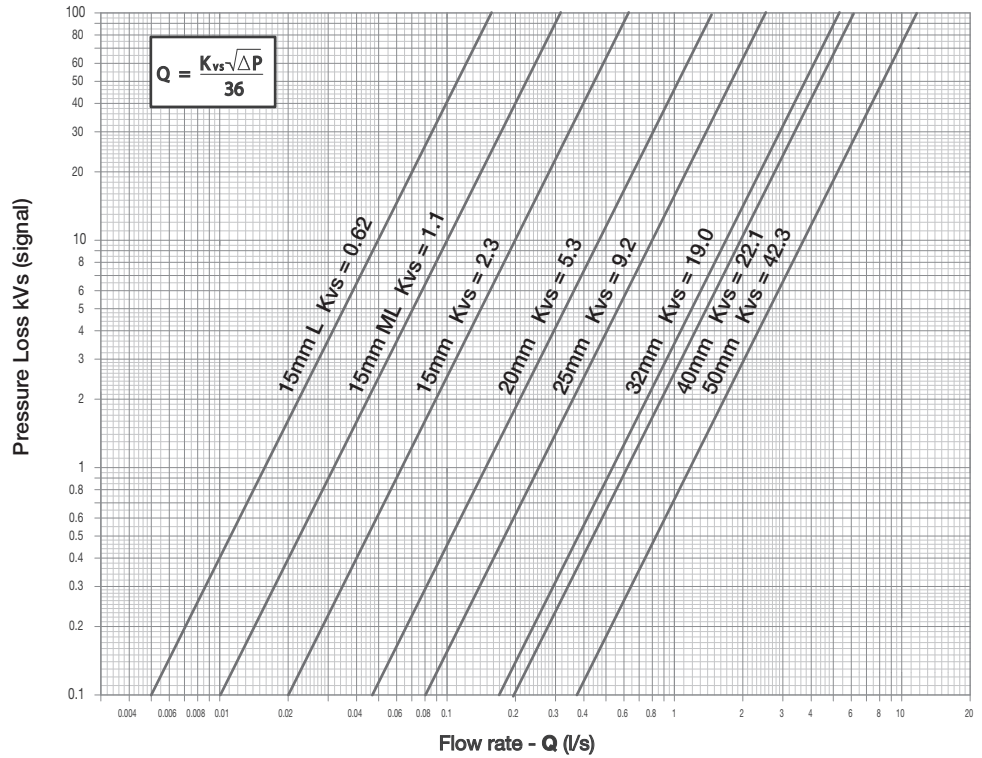
Kvs (Flow rate in m 3 /h @ 1 bar pressure drop)
